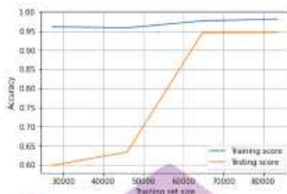
Gambar 4. 15 Learning Curve Analyst Wordnet Lemmatizer dan BoW Dataset 1
