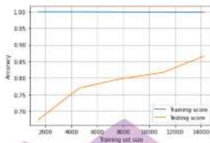
Gambar 4. 18 Learning Curve Analyst SnowBall Stemmer dan N-Gram Dataset 2
