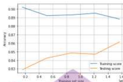
Gambar 4. 27 Learning Curve Analyst Wordnet Lemmatizer dan BoW Dataset 3
