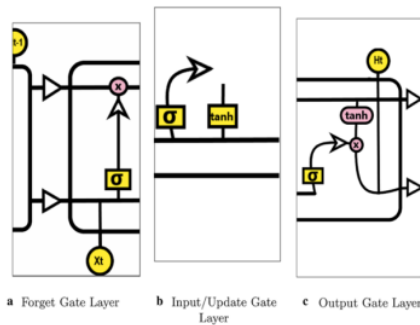
Figure. 4 Basic mechanism of LSTM network [30]
