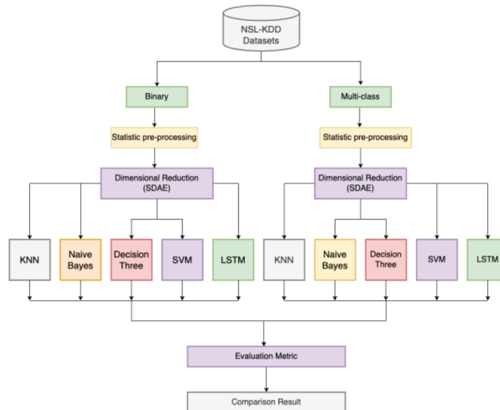
Figure. 2 Scenario of IDS network attack detection experiment
