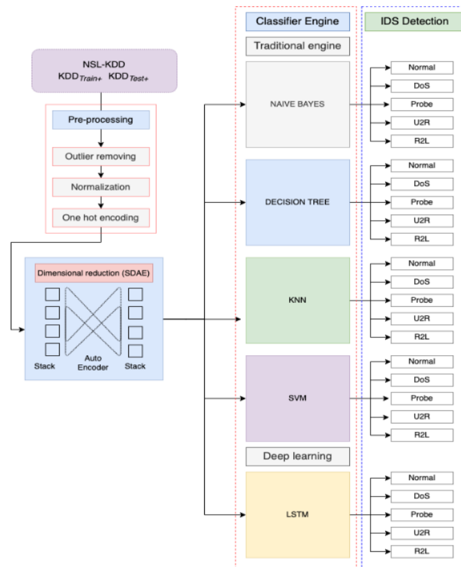
Figure. 5 Proposed model of SDAE & traditional machine
