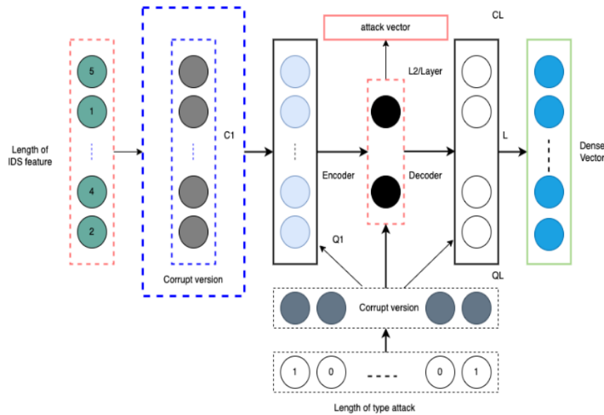
Figure. 3 SDAE framework for dimensional reduction
