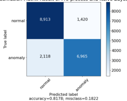
Confusion Matrix Result of Pre-process and Naive Bayes
