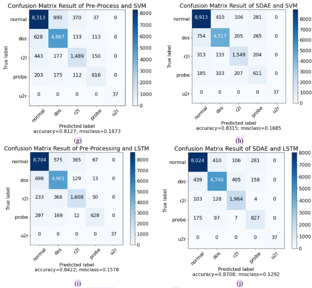
Figure. 8 Experiment scenario for multi-class classification
