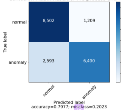
Confusion Matrix Result of Pre-process and Naive Bayes
