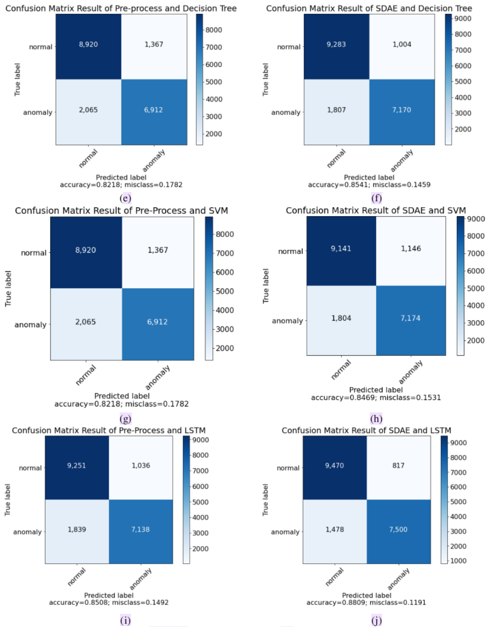
Figure. 7 Experiment scenario for binary classification
